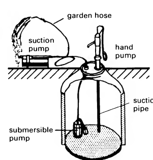
11 Rainwater storage for garden watering
